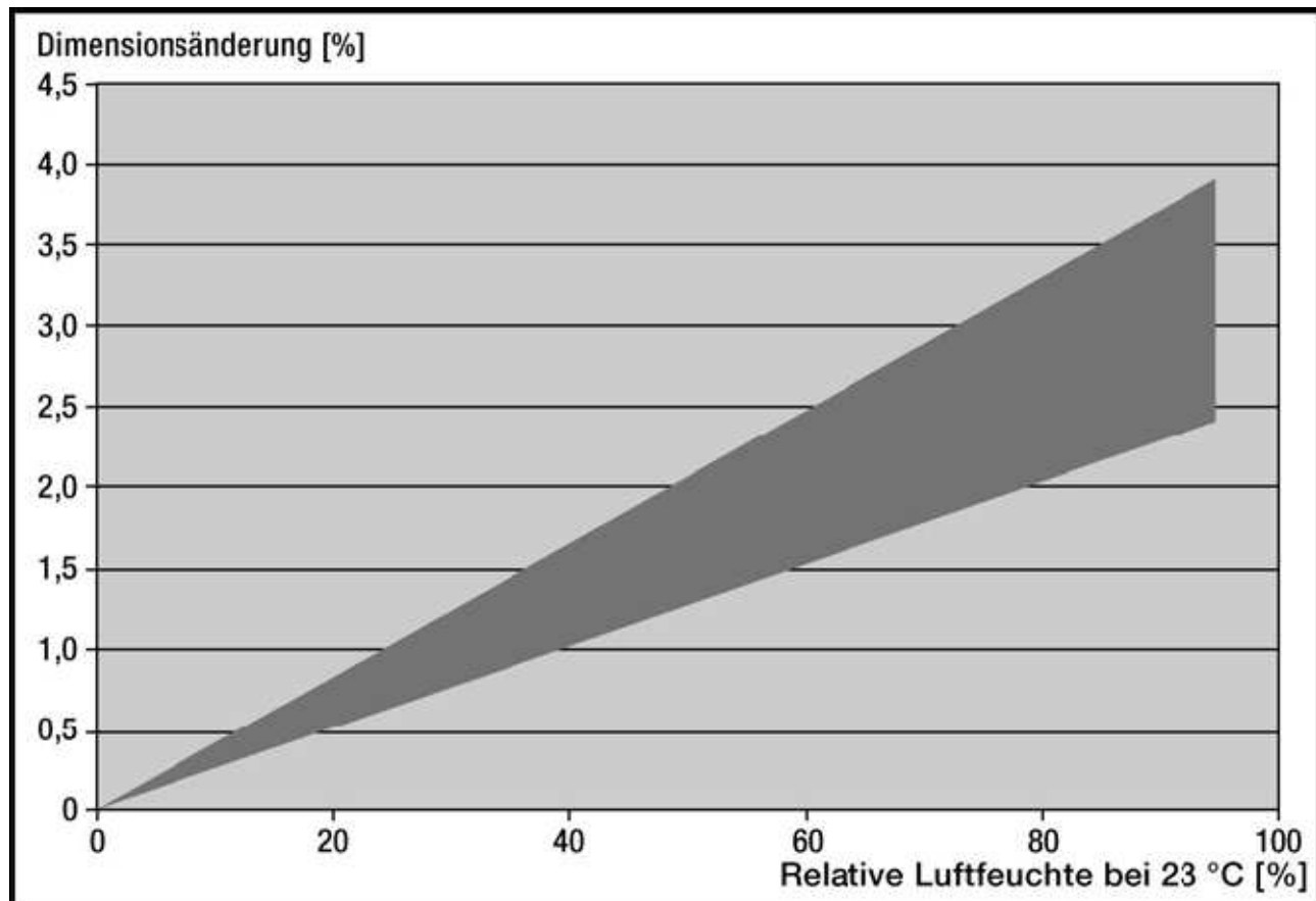
Diagram 1: Dimensional change subject to the relative room air humidity at an ambient temperature of 23°C
