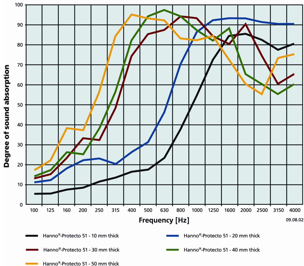
Measurement according to DIN-EN-ISO 10534-2 impedance tube
